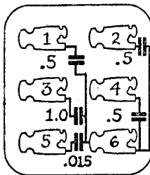
Internal Connections Filter Condenser
